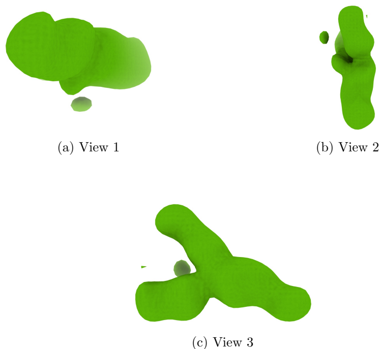
Figure 4: Isosurface at threshold=3.390000. Views generated by ChimeraX at a the following X, Y, Z angles: View 1 (0, -90, -90), View 2 (-90, 0, -90), View 3 (0, 0, 0).
