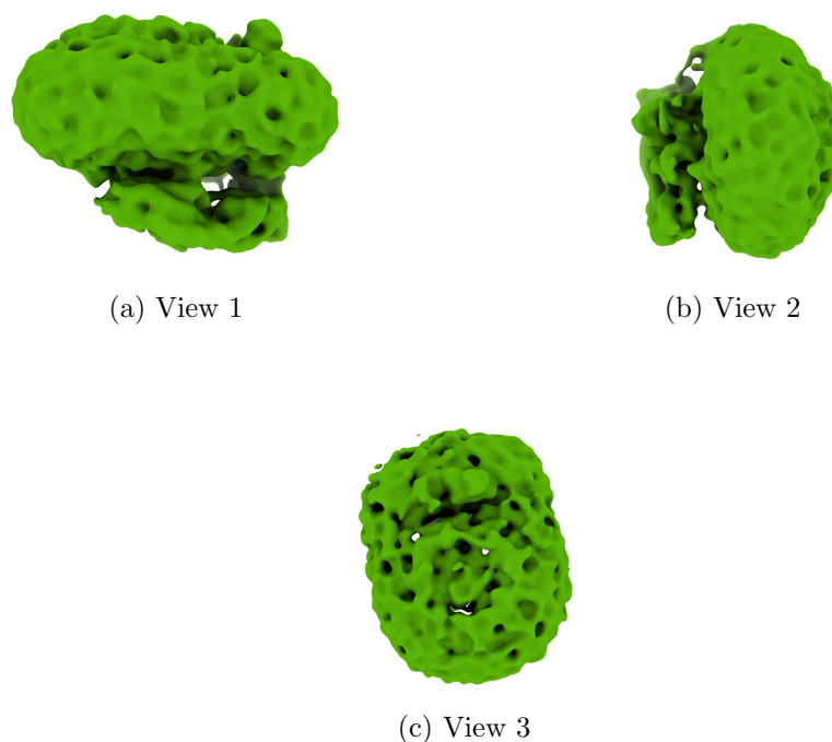
Figure 4: Isosurface at threshold=0.044500. Views generated by ChimeraX at a the following X, Y, Z angles: View 1 (0, -90, -90), View 2 (-90, 0, -90), View 3 (0, 0, 0).
