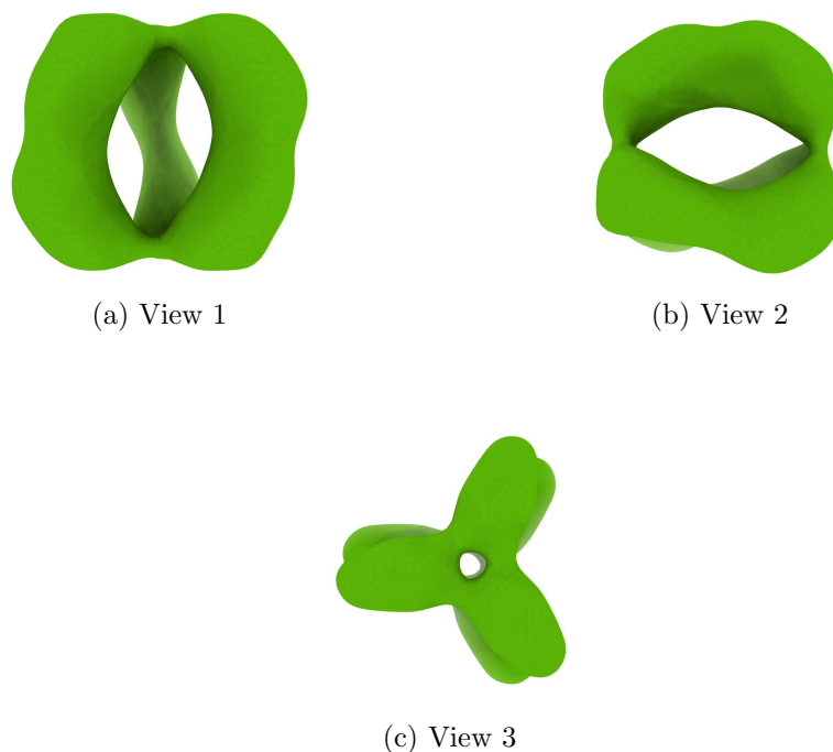
Figure 4: Isosurface at threshold=1.280000. Views generated by ChimeraX at a the following X, Y, Z angles: View 1 (0, -90, -90), View 2 (-90, 0, -90), View 3 (0, 0, 0).
