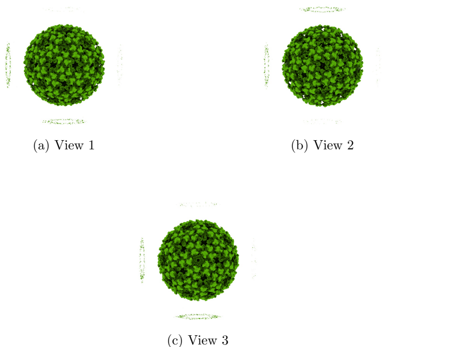
Figure 4: Isosurface at threshold=0.700000. Views generated by ChimeraX at the following X, Y, Z angles: View 1 (0, -90, -90), View 2 (-90, 0, -90), View 3 (0, 0, 0).
