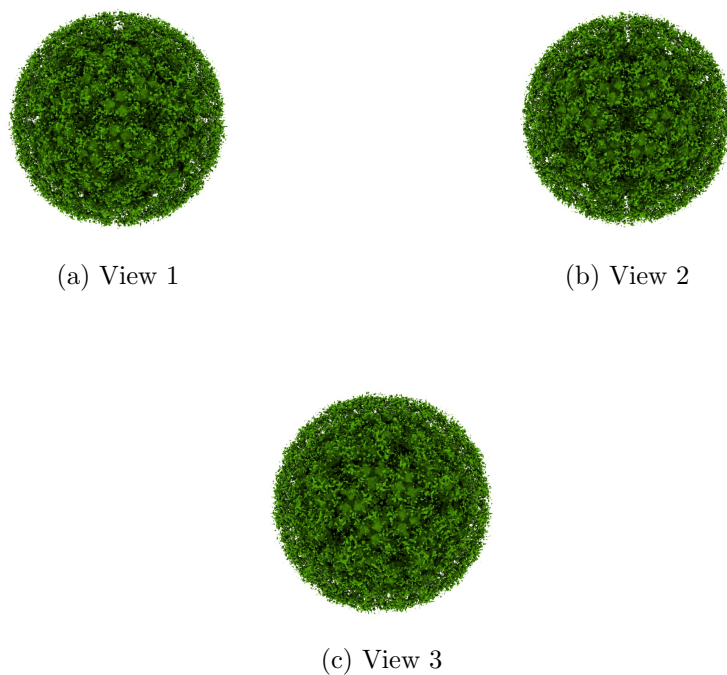
Figure 4: Isosurface at threshold=0.630000. Views generated by ChimeraX at a the following X, Y, Z angles: View 1 (0, -90, -90), View 2 (-90, 0, -90), View 3 (0, 0, 0).
