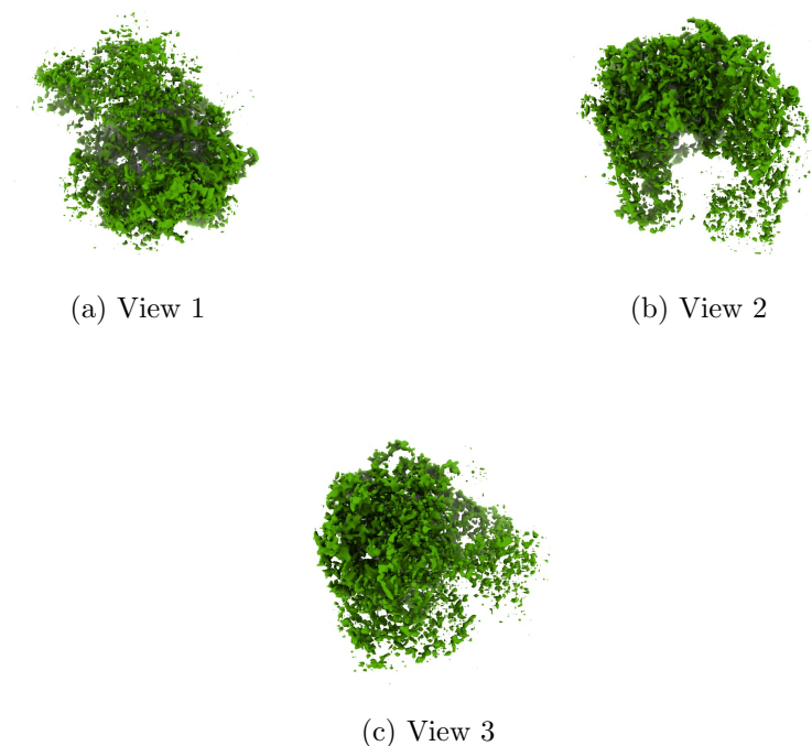
Figure 4: Isosurface at threshold=0.043600. Views generated by ChimeraX at a the following X, Y, Z angles: View 1 (0, -90, -90), View 2 (-90, 0, -90), View 3 (0, 0, 0).
