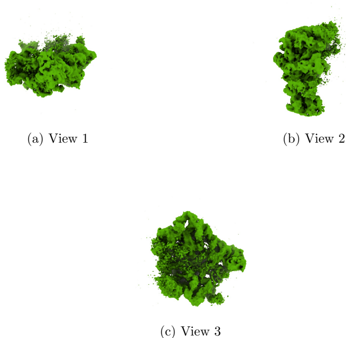
Figure 4: Isosurface at threshold=0.027200. Views generated by ChimeraX at a the following X, Y, Z angles: View 1 (0, -90, -90), View 2 (-90, 0, -90), View 3 (0, 0, 0).
