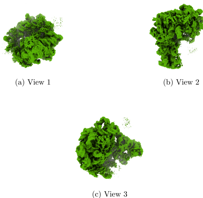
Figure 4: Isosurface at threshold=0.030400. Views generated by ChimeraX at a the following X, Y, Z angles: View 1 (0, -90, -90), View 2 (-90, 0, -90), View 3 (0, 0, 0).
