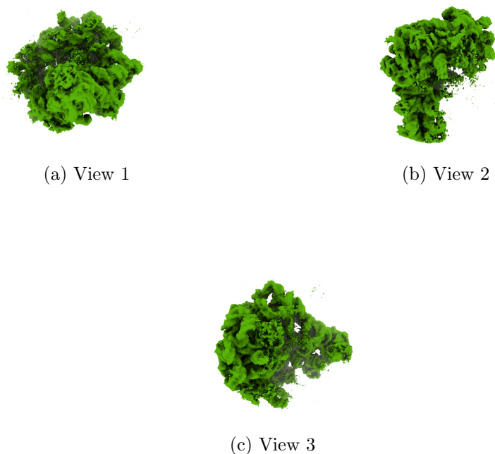
Figure 4: Isosurface at threshold=0.030300. Views generated by ChimeraX at a the following X, Y, Z angles: View 1 (0, -90, -90), View 2 (-90, 0, -90), View 3 (0, 0, 0).
