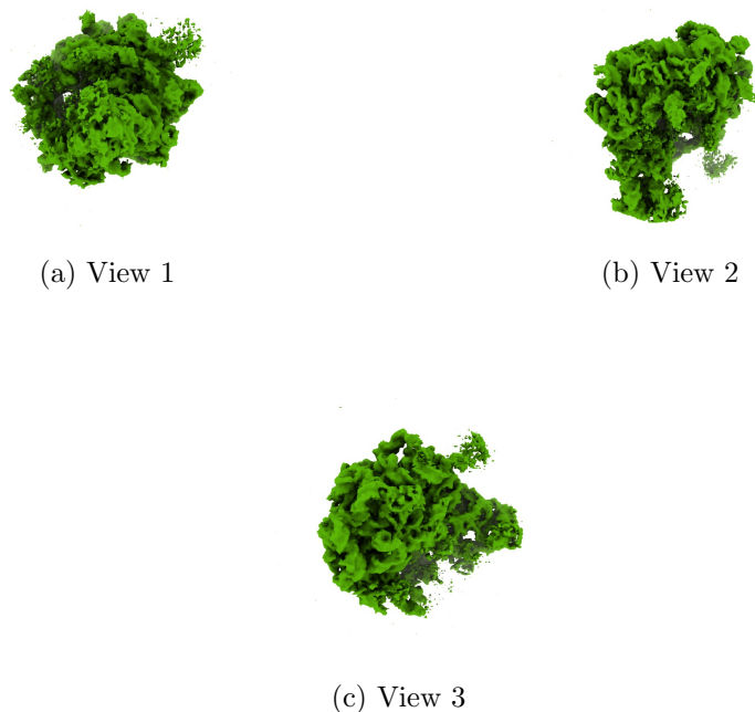
Figure 4: Isosurface at threshold=0.034400. Views generated by ChimeraX at a the following X, Y, Z angles: View 1 (0, -90, -90), View 2 (-90, 0, -90), View 3 (0, 0, 0).
