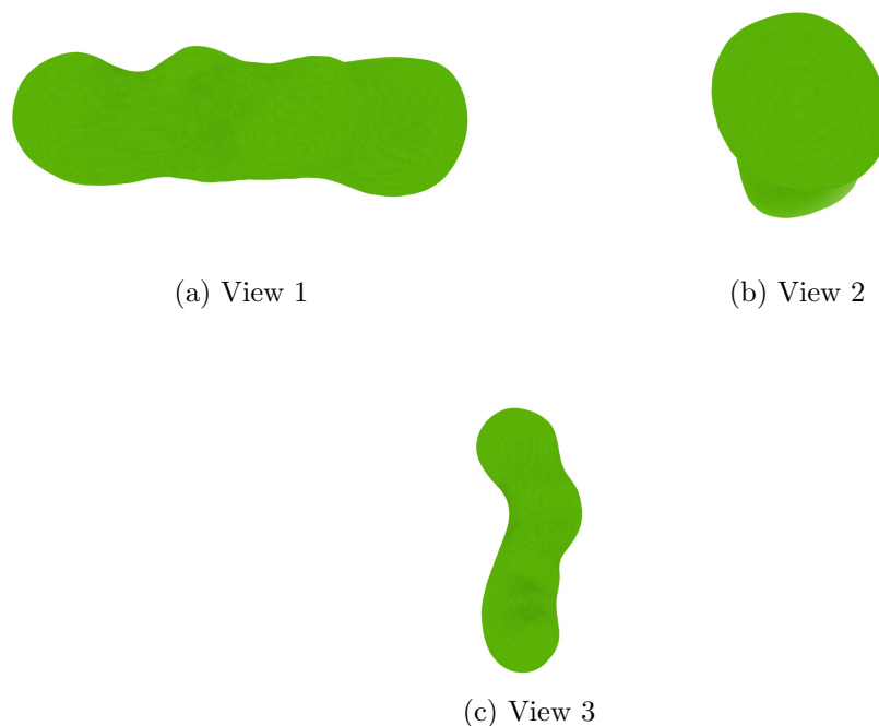
Figure 4: Isosurface at threshold=0.099800. Views generated by ChimeraX at a the following X, Y, Z angles: View 1 (0, -90, -90), View 2 (-90, 0, -90), View 3 (0, 0, 0).
