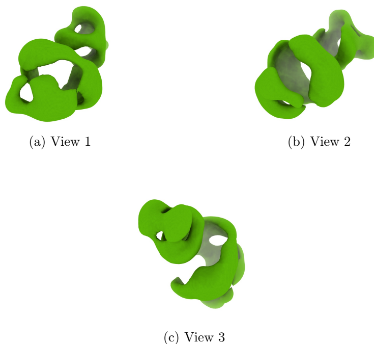
Figure 4: Isosurface at threshold=0.029200. Views generated by ChimeraX at a the following X, Y, Z angles: View 1 (0, -90, -90), View 2 (-90, 0, -90), View 3 (0, 0, 0).
