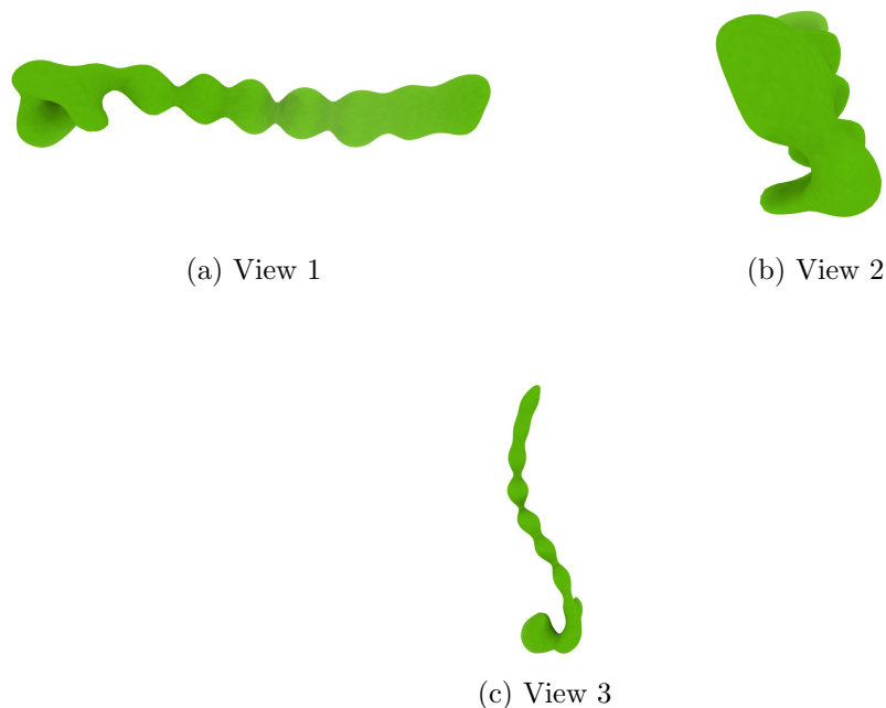
Figure 4: Isosurface at threshold=0.052600. Views generated by ChimeraX at a the following X, Y, Z angles: View 1 (0, -90, -90), View 2 (-90, 0, -90), View 3 (0, 0, 0).
