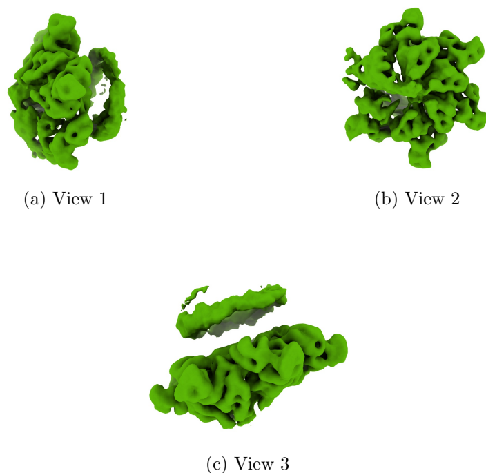
Figure 4: Isosurface at threshold=0.019700. Views generated by ChimeraX at a the following X, Y, Z angles: View 1 (0, -90, -90), View 2 (-90, 0, -90), View 3 (0, 0, 0).
