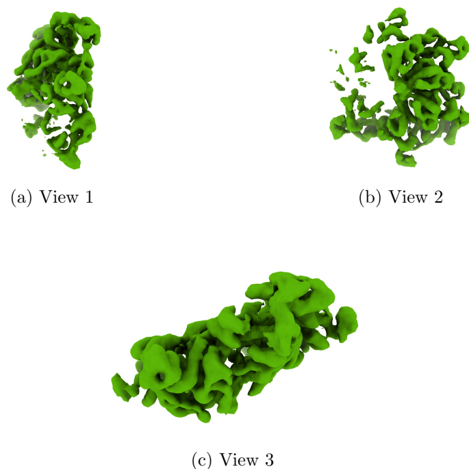
Figure 4: Isosurface at threshold=0.025300. Views generated by ChimeraX at a the following X, Y, Z angles: View 1 (0, -90, -90), View 2 (-90, 0, -90), View 3 (0, 0, 0).
