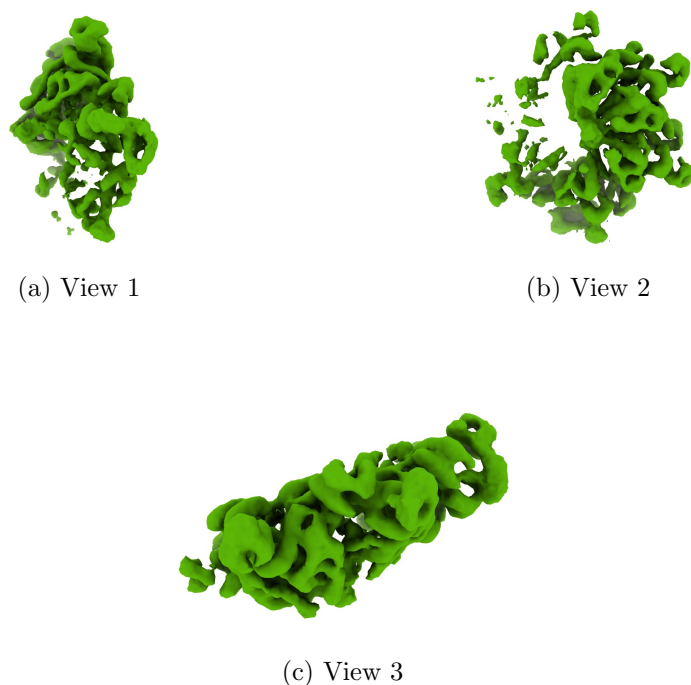
Figure 4: Isosurface at threshold=0.025200. Views generated by ChimeraX at a the following X, Y, Z angles: View 1 (0, -90, -90), View 2 (-90, 0, -90), View 3 (0, 0, 0).
