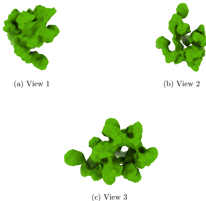
Figure 4: Isosurface at threshold=0.001500. Views generated by ChimeraX at a the following X, Y, Z angles: View 1 (0, -90, -90), View 2 (-90, 0, -90), View 3 (0, 0, 0).
