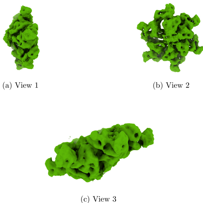
Figure 4: Isosurface at threshold=0.021200. Views generated by ChimeraX at a the following X, Y, Z angles: View 1 (0, -90, -90), View 2 (-90, 0, -90), View 3 (0, 0, 0).
