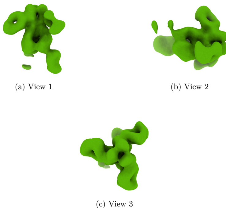
Figure 4: Isosurface at threshold=20.700000. Views generated by ChimeraX at a the following X, Y, Z angles: View 1 (0, -90, -90), View 2 (-90, 0, -90), View 3 (0, 0, 0).
