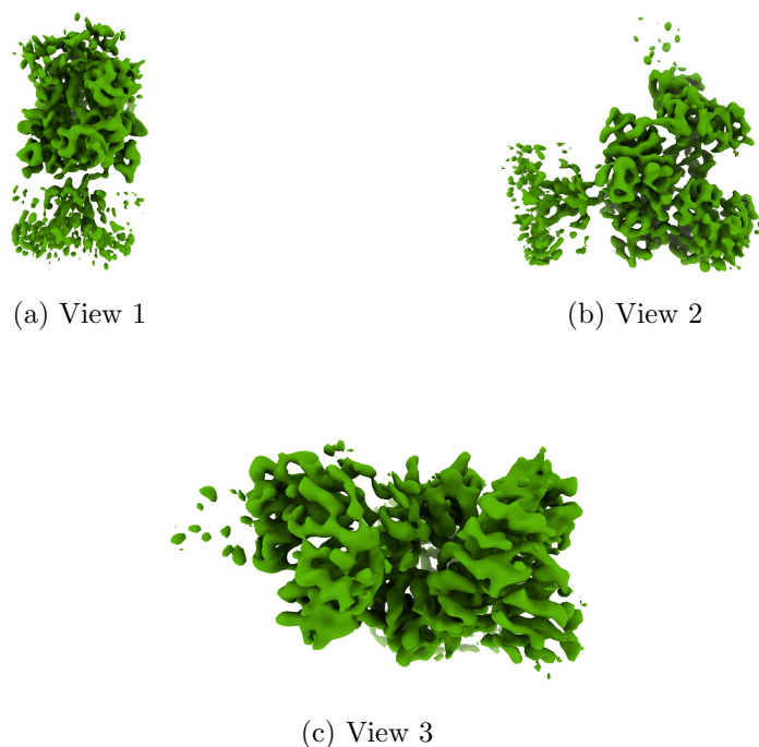
Figure 4: Isosurface at threshold=0.240000. Views generated by ChimeraX at a the following X, Y, Z angles: View 1 (0, -90, -90), View 2 (-90, 0, -90), View 3 (0, 0, 0).
