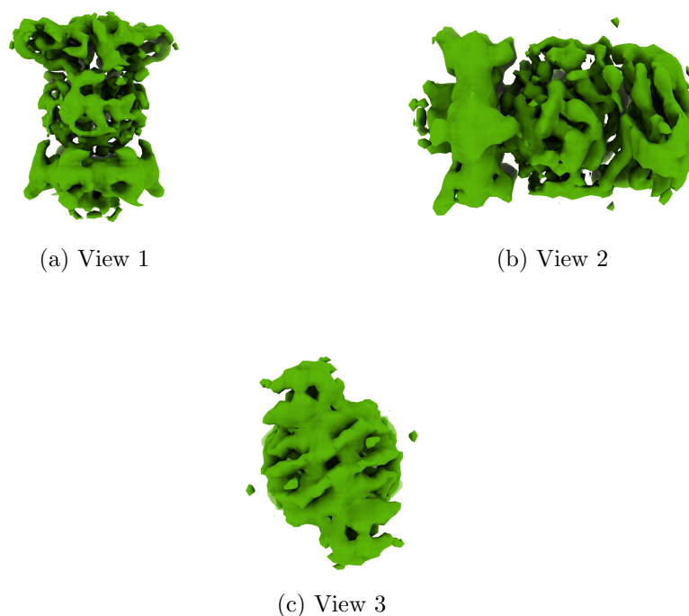
Figure 4: Isosurface at threshold=0.139000. Views generated by ChimeraX at a the following X, Y, Z angles: View 1 (0, -90, -90), View 2 (-90, 0, -90), View 3 (0, 0, 0).
