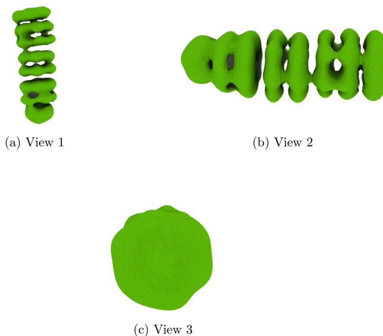
Figure 4: Isosurface at threshold=0.086000. Views generated by ChimeraX at a the following X, Y, Z angles: View 1 (0, -90, -90), View 2 (-90, 0, -90), View 3 (0, 0, 0).
