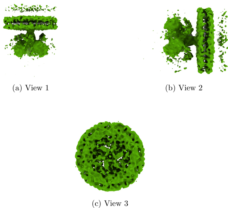
Figure 4: Isosurface at threshold=0.002320. Views generated by ChimeraX at a the following X, Y, Z angles: View 1 (0, -90, -90), View 2 (-90, 0, -90), View 3 (0, 0, 0).
