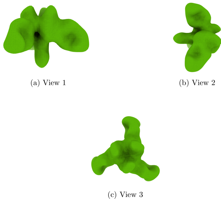
Figure 4: Isosurface at threshold=2.660000. Views generated by ChimeraX at a the following X, Y, Z angles: View 1 (0, -90, -90), View 2 (-90, 0, -90), View 3 (0, 0, 0).
