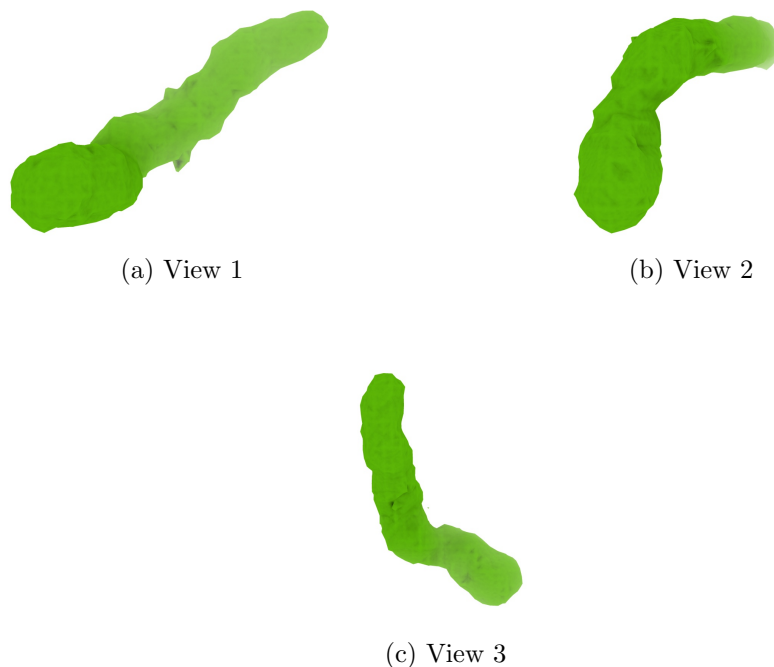
Figure 4: Isosurface at threshold=4.600000. Views generated by ChimeraX at a the following X, Y, Z angles: View 1 (0, -90, -90), View 2 (-90, 0, -90), View 3 (0, 0, 0).
