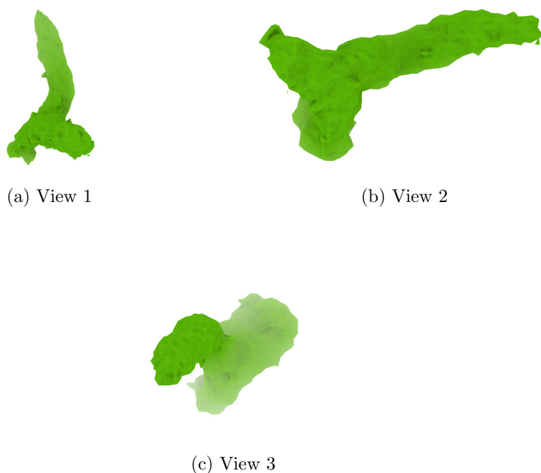
Figure 4: Isosurface at threshold=4.790000. Views generated by ChimeraX at a the following X, Y, Z angles: View 1 (0, -90, -90), View 2 (-90, 0, -90), View 3 (0, 0, 0).
