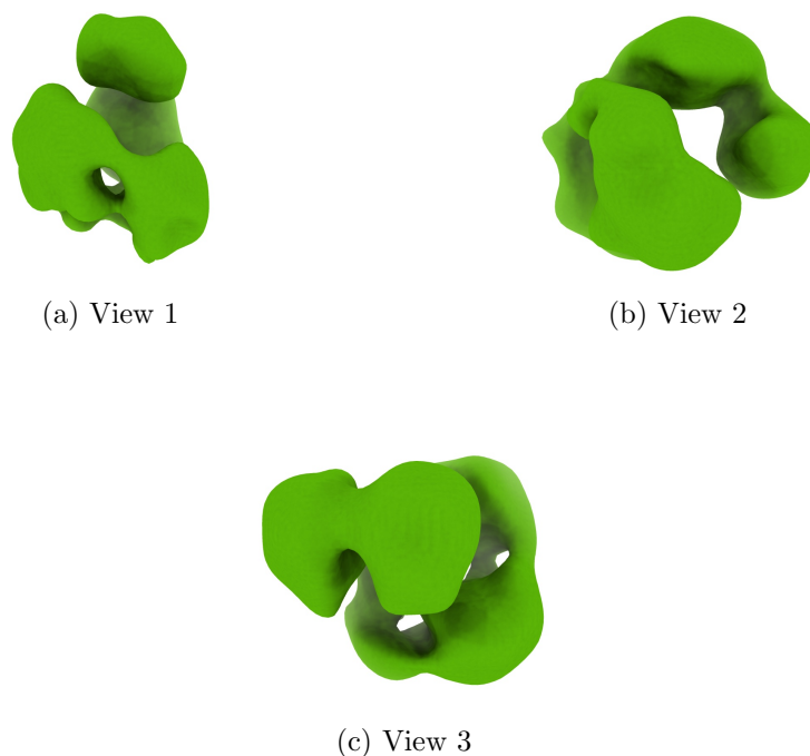
Figure 4: Isosurface at threshold=1.380000. Views generated by ChimeraX at a the following X, Y, Z angles: View 1 (0, -90, -90), View 2 (-90, 0, -90), View 3 (0, 0, 0).
