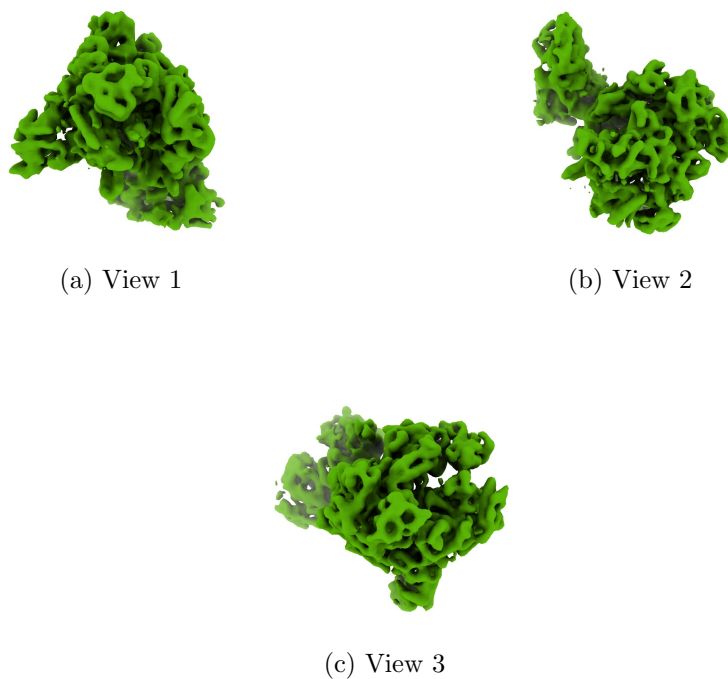
Figure 4: Isosurface at threshold=0.070000. Views generated by ChimeraX at a the following X, Y, Z angles: View 1 (0, -90, -90), View 2 (-90, 0, -90), View 3 (0, 0, 0).
