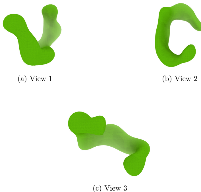
Figure 4: Isosurface at threshold=0.058900. Views generated by ChimeraX at a the following X, Y, Z angles: View 1 (0, -90, -90), View 2 (-90, 0, -90), View 3 (0, 0, 0).
