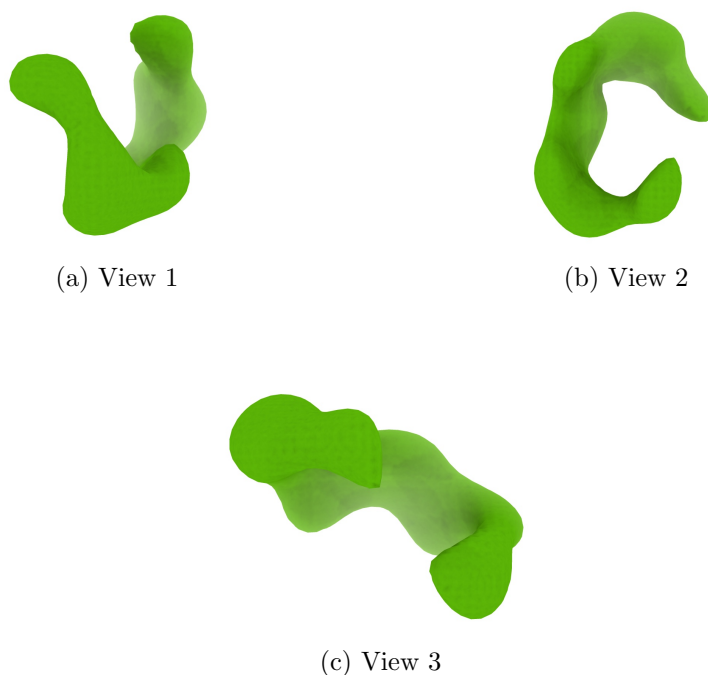
Figure 4: Isosurface at threshold=0.622000. Views generated by ChimeraX at a the following X, Y, Z angles: View 1 (0, -90, -90), View 2 (-90, 0, -90), View 3 (0, 0, 0).
