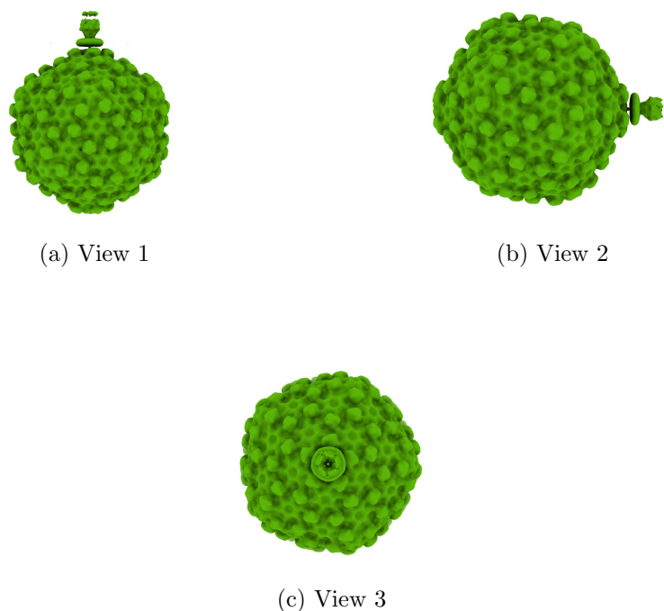
Figure 4: Isosurface at threshold=48.400000. Views generated by ChimeraX at a the following X, Y, Z angles: View 1 (0, -90, -90), View 2 (-90, 0, -90), View 3 (0, 0, 0).
