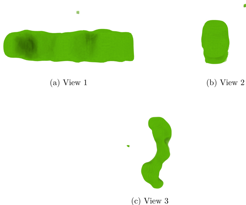
Figure 4: Isosurface at threshold=0.020000. Views generated by ChimeraX at a the following
