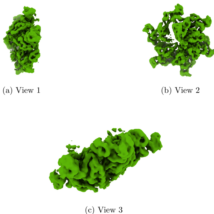
Figure 4: Isosurface at threshold=0.013100. Views generated by ChimeraX at a the following X, Y, Z angles: View 1 (0, -90, -90), View 2 (-90, 0, -90), View 3 (0, 0, 0).
