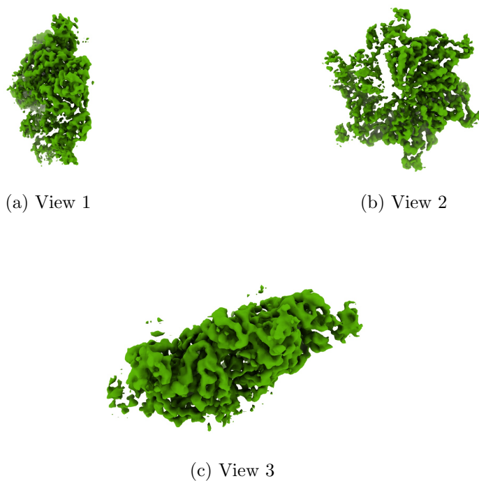
Figure 4: Isosurface at threshold=0.019700. Views generated by ChimeraX at a the following X, Y, Z angles: View 1 (0, -90, -90), View 2 (-90, 0, -90), View 3 (0, 0, 0).
