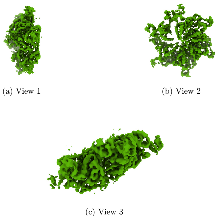
Figure 4: Isosurface at threshold=0.020400. Views generated by ChimeraX at a the following X, Y, Z angles: View 1 (0, -90, -90), View 2 (-90, 0, -90), View 3 (0, 0, 0).
