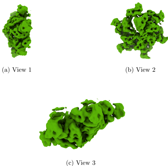
Figure 4: Isosurface at threshold=0.010800. Views generated by ChimeraX at a the following X, Y, Z angles: View 1 (0, -90, -90), View 2 (-90, 0, -90), View 3 (0, 0, 0).
