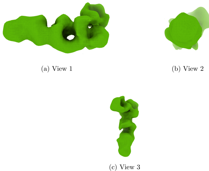
Figure 4: Isosurface at threshold=4.630000. Views generated by ChimeraX at a the following X, Y, Z angles: View 1 (0, -90, -90), View 2 (-90, 0, -90), View 3 (0, 0, 0).
