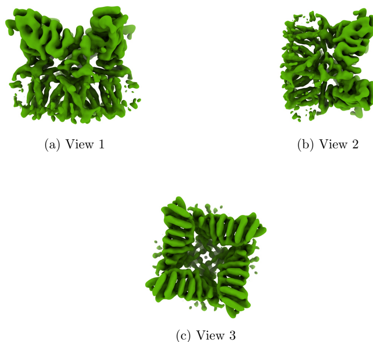
Figure 4: Isosurface at threshold=0.026800. Views generated by ChimeraX at a the following X, Y, Z angles: View 1 (0, -90, -90), View 2 (-90, 0, -90), View 3 (0, 0, 0).
