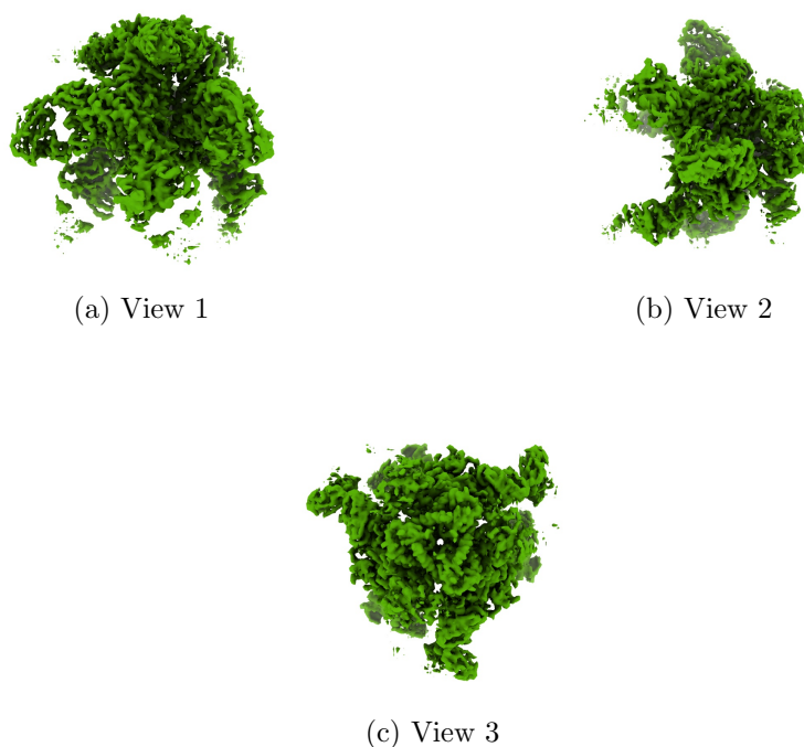
Figure 4: Isosurface at threshold=1.640000. Views generated by ChimeraX at a the following X, Y, Z angles: View 1 (0, -90, -90), View 2 (-90, 0, -90), View 3 (0, 0, 0).
