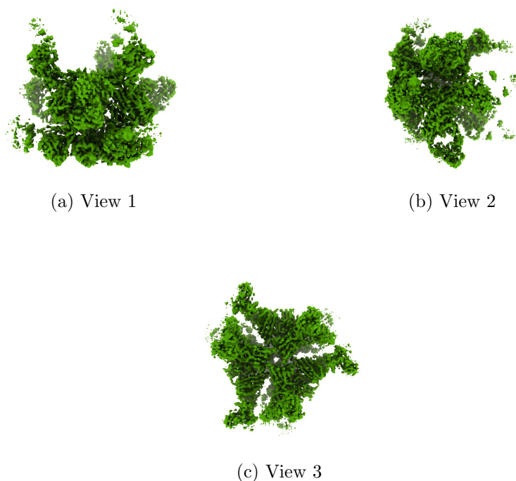
Figure 4: Isosurface at threshold=1.190000. Views generated by ChimeraX at a the following X, Y, Z angles: View 1 (0, -90, -90), View 2 (-90, 0, -90), View 3 (0, 0, 0).
