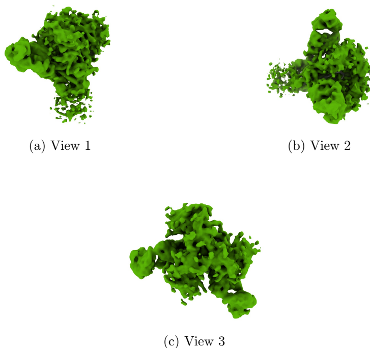
Figure 4: Isosurface at threshold=0.023400. Views generated by ChimeraX at a the following X, Y, Z angles: View 1 (0, -90, -90), View 2 (-90, 0, -90), View 3 (0, 0, 0).
