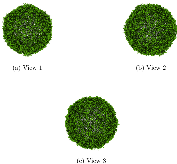
Figure 4: Isosurface at threshold=36.400000. Views generated by ChimeraX at a the following X, Y, Z angles: View 1 (0, -90, -90), View 2 (-90, 0, -90), View 3 (0, 0, 0).
