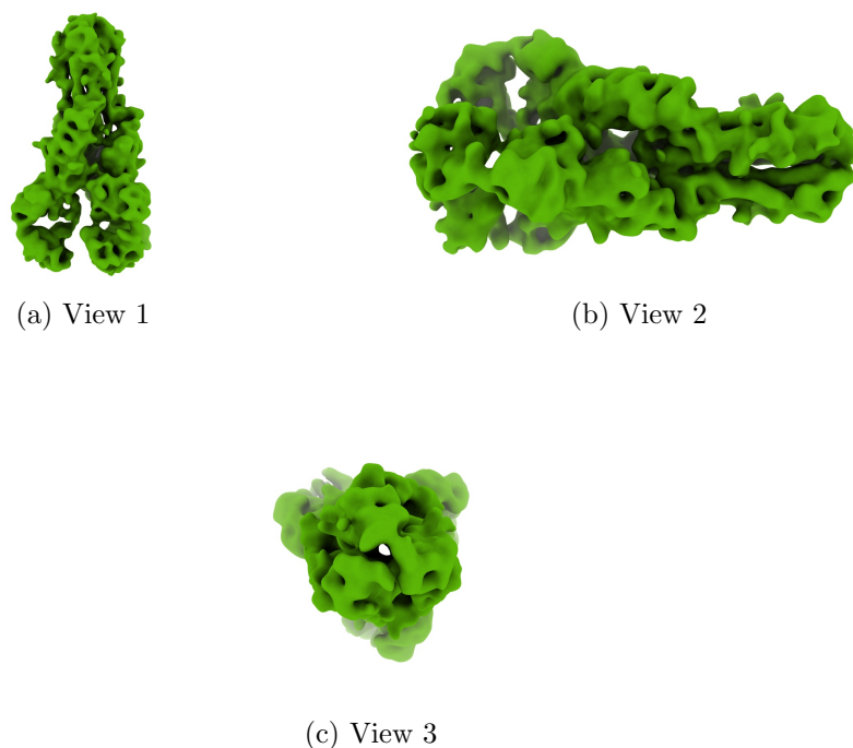
Figure 4: Isosurface at threshold=0.027400. Views generated by ChimeraX at the following X, Y, Z angles: View 1 (0, -90, -90), View 2 (-90, 0, -90), View 3 (0, 0, 0).
