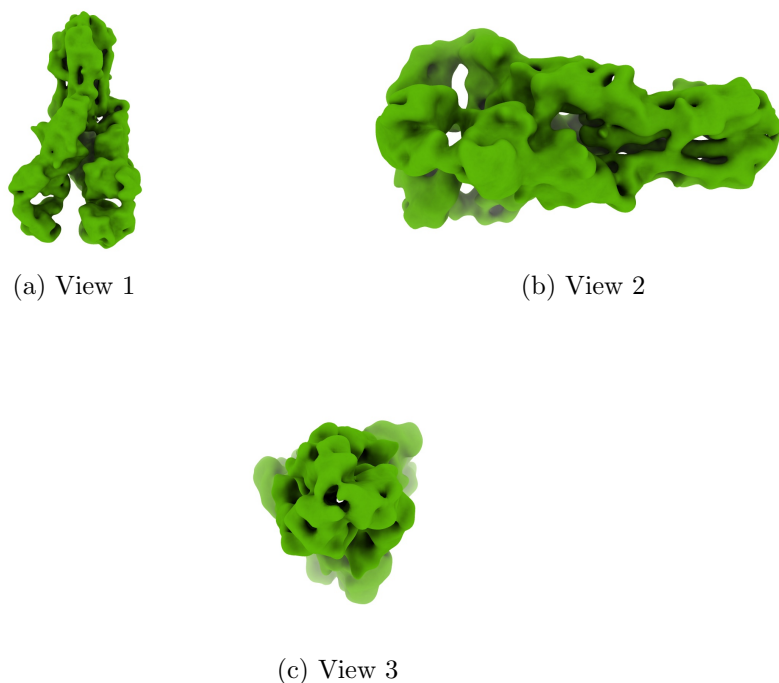
Figure 4: Isosurface at threshold=0.033400. Views generated by ChimeraX at a the following X, Y, Z angles: View 1 (0, -90, -90), View 2 (-90, 0, -90), View 3 (0, 0, 0).
