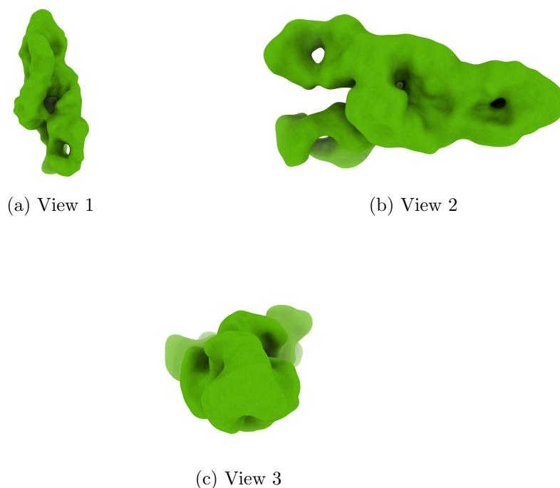
Figure 4: Isosurface at threshold=0.035000. Views generated by ChimeraX at a the following X, Y, Z angles: View 1 (0, -90, -90), View 2 (-90, 0, -90), View 3 (0, 0, 0).
