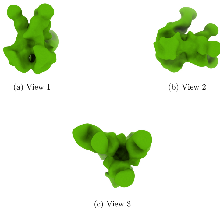
Figure 4: Isosurface at threshold=0.018100. Views generated by ChimeraX at a the following X, Y, Z angles: View 1 (0, -90, -90), View 2 (-90, 0, -90), View 3 (0, 0, 0).
