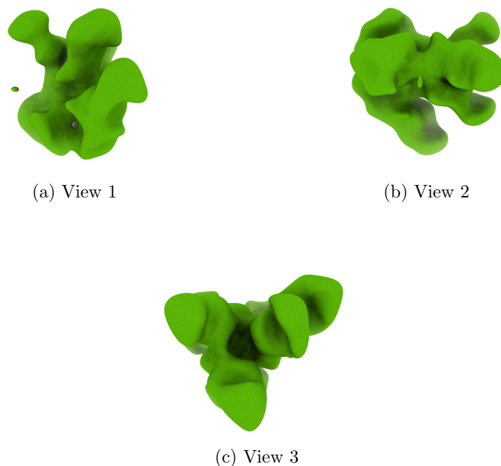
Figure 4: Isosurface at threshold=0.013400. Views generated by ChimeraX at a the following X, Y, Z angles: View 1 (0, -90, -90), View 2 (-90, 0, -90), View 3 (0, 0, 0).
