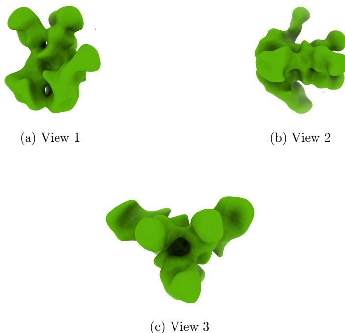
Figure 4: Isosurface at threshold=0.015200. Views generated by ChimeraX at a the following X, Y, Z angles: View 1 (0, -90, -90), View 2 (-90, 0, -90), View 3 (0, 0, 0).
