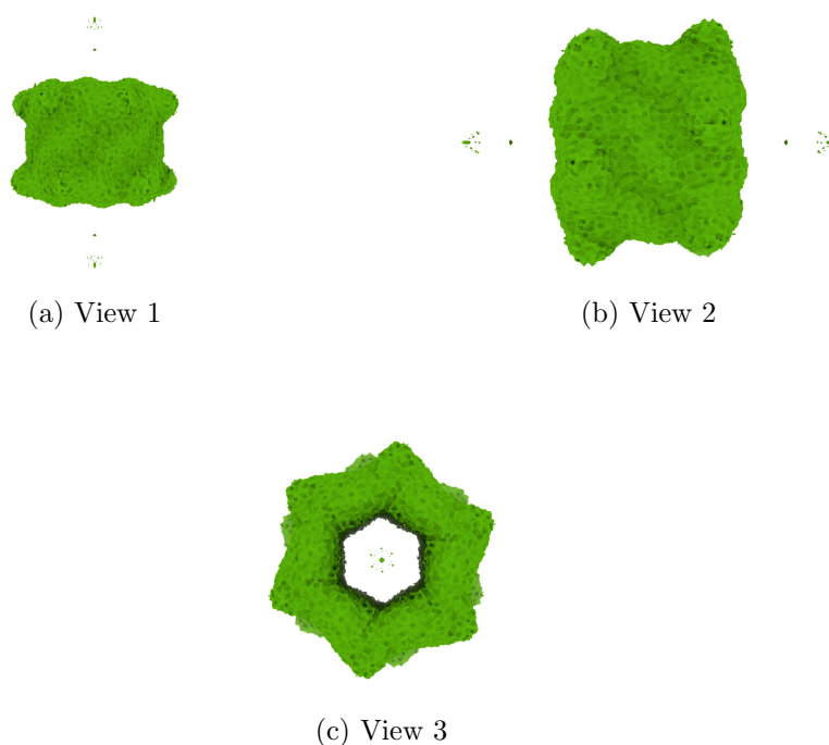
Figure 4: Isosurface at threshold=0.368000. Views generated by ChimeraX at a the following X, Y, Z angles: View 1 (0, -90, -90), View 2 (-90, 0, -90), View 3 (0, 0, 0).
