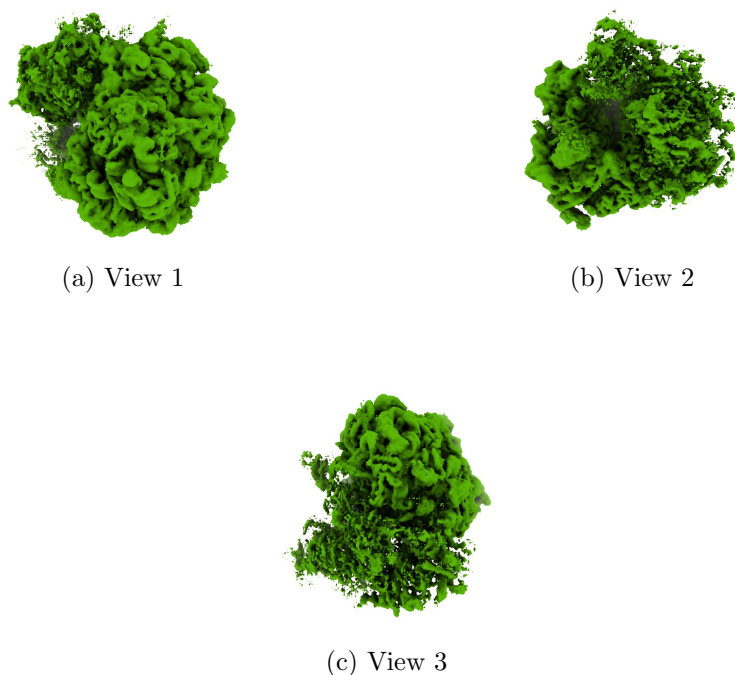
Figure 4: Isosurface at threshold=0.592000. Views generated by ChimeraX at a the following X, Y, Z angles: View 1 (0, -90, -90), View 2 (-90, 0, -90), View 3 (0, 0, 0).
